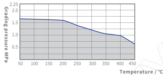
WCB/A105 material PN16 Valve body pressure-temperature ratings
