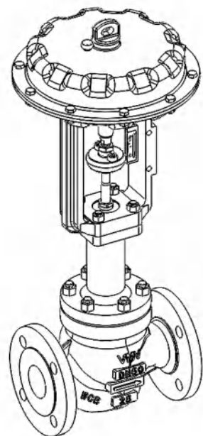
Pneumatic bellows conventional structure
