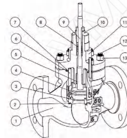
Conventional control valve
