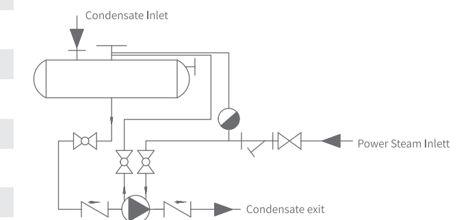
Flow Chart of Single Pump Trap System
