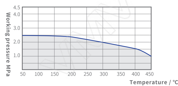
WCB/A105 material PN25 Valve body pressure-temperature ratings
