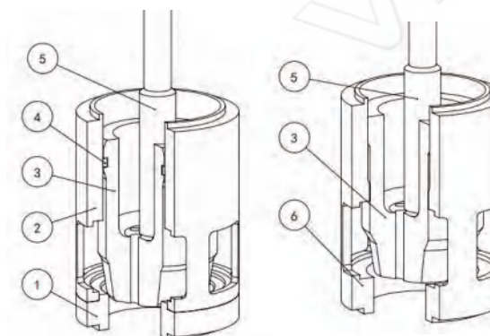
Balanced single-seat structure Balanced double-seat structure
