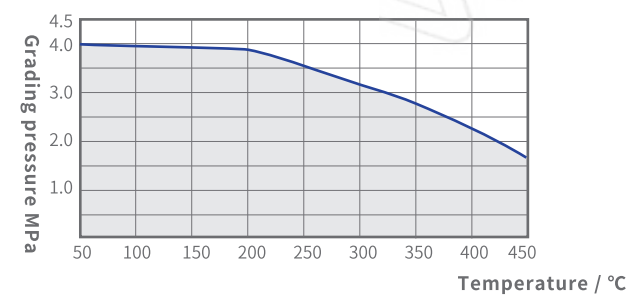
WCB/A105 material PN40 Valve body pressure-temperature ratings
