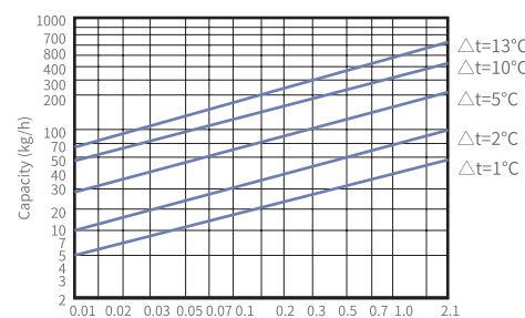
Differential Pressure (MPa) ▲t= Setting temperature-Valve actual drainage temperature
