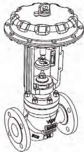
Pneumatic conventional structure
