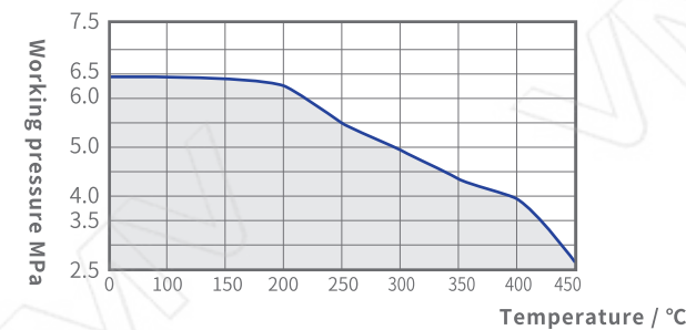
WCB/A105 material PN63 Valve body pressure-temperature ratings
