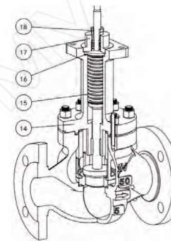
Bellows control valve
